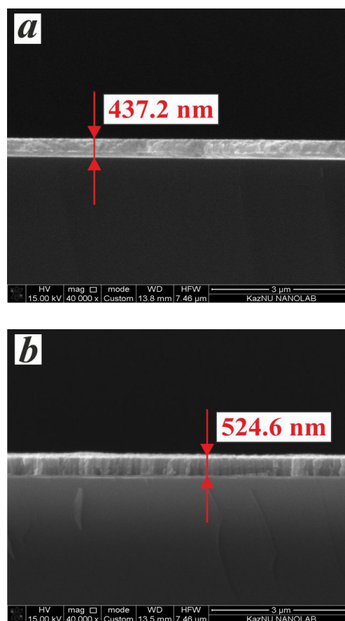
Fig. 1. Cross SEM image of thin copper film on a silicon substrate: a – 30 min, b – 60 min.
